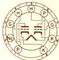
BOTTOM VIEW MINIATURE BUTTON 9 PIN BASE 9EF
