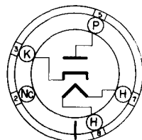
BOTTOM VIEW A
