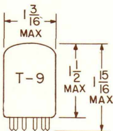
GLASS BULB 9-62
