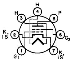
BOTTOM VIEW BASING DIAGRAM JEDEC 7EW
