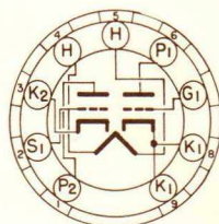
BOTTOM VIEW SMALL BUTTON 9 PIN BASE 9FC
