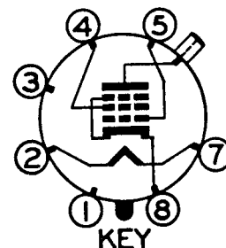
RETMA 6AM
