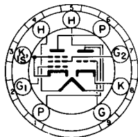
BOTTOM VIEW MINIATURE BUTTON 9 PIN BASE 9FZ
