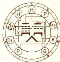
BOTTOM VIEW MINIATURE BUTTON 9 PIN BASE 9FZ
