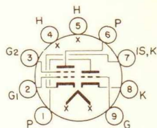
BOTTOM VIEW BASING DIAGRAM JEDEC 9CE
