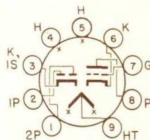
BOTTOM VIEW BASING DIAGRAM
