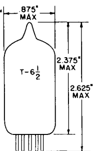
GLASS BULB SMALL BUTTON NOVAL 9 PIN BASE E9-1 OUTLINE DRAWING JEDEC 6-3
