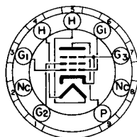
BOTTOM VIEW MINIATURE BUTT 9 PIN BASE 9CK
