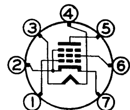
RETMA 7BD
