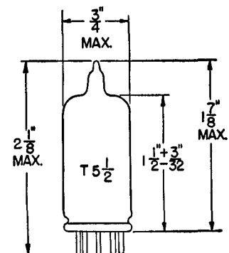
RETMA 5-2
