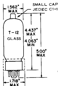
OUTLINE DRAWING JEDEC 12-36
