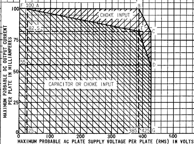
RATING CHART I 6CA4
