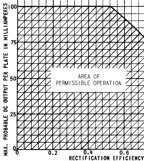
RATING CHART II 6CA4
