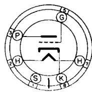
BOTTOM VIEW 6C5 6C5GT
