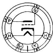
BOTTOM VIEW 6C5G
