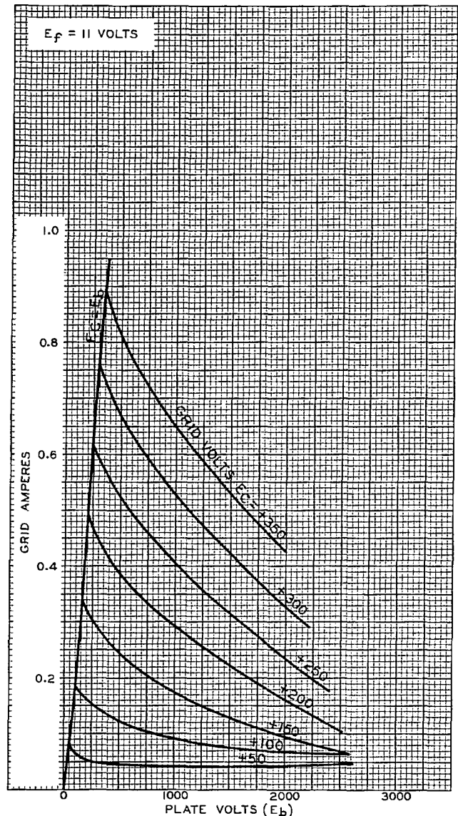
Fig. 6 - Typical Grid Characteristics.
