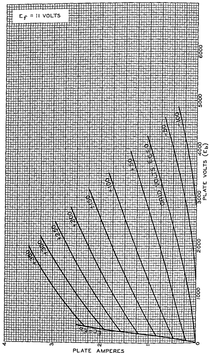
Fig. 5 - Average Plate Characteristics.
