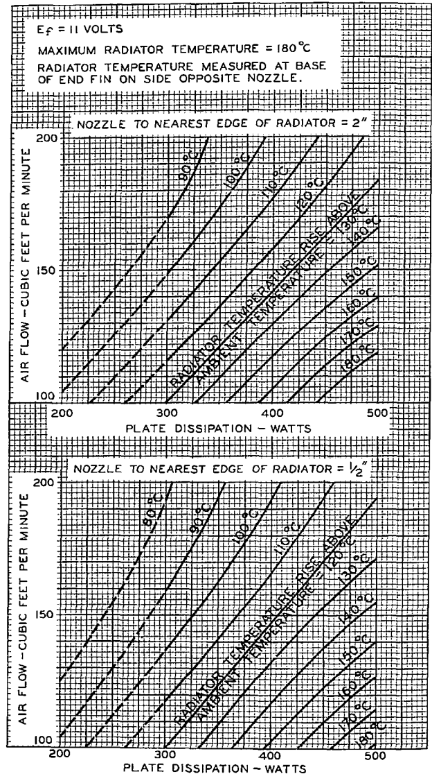
Fig. 2 - Cooling Requirements for Method I.
