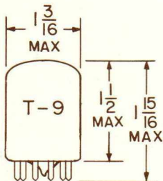
GLASS BULB
