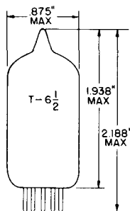
GLASS BULB MINIATURE BUTT 9 PIN BASE E9-1 OUTLINE DRAWING JEDEC 6-2
