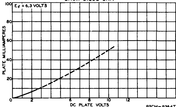
AVERAGE PLATE CHARACTERISTIC EACH DIODE UNIT
