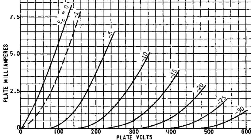
6BN7 SECTION #2 E_f = 6.3 Volts
