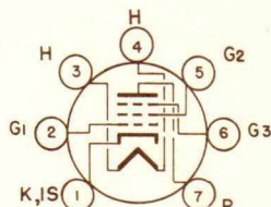
BOTTOM VIEW BASING DIAGRAM JEDEC 70F
