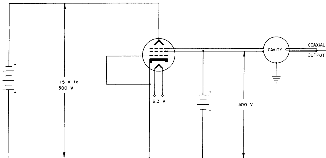
FIG. 1 — CW OSCILLATOR CIRCUIT EMPLOYING THE 6BL6 REFLEX KLYSTRON
