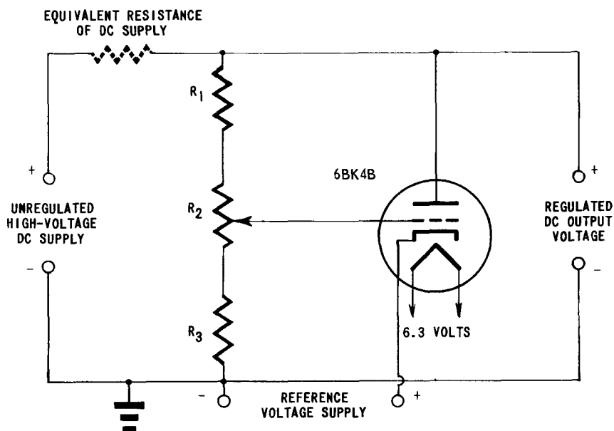
SHUNT VOLTAGE-REGULATOR CIRCUIT
