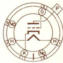
BOTTOM VIEW SHORT JUMBO-SHELL 6 PIN OCTAL
