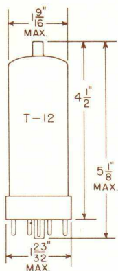
GLASS BULB SMALL CAP
