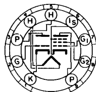
BOTTOM VIEW MINIATURE BOTTOM 9 PIN BASE 90°
