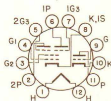
BOTTOM VIEW BASING DIAGRAM JEDEC 12ER
