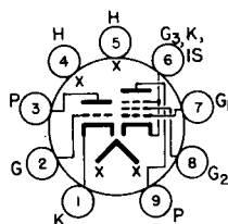
BOTTOM VIEW BASING DIAGRAM JEDEC 9DX
