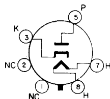
BOTTOM VIEW PINING DIAGRAM JEDEC 4CG
