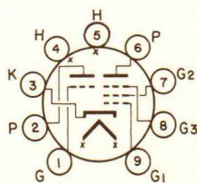
BOTTOM VIEW BASING DIAGRAM JEDEC 9DW
