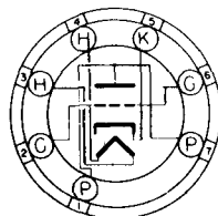
BOTTOM VIEW MINIATURE BUTTON 7 PIN BASE 70K
