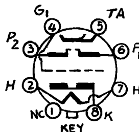
Bottom View of Socket Connections
