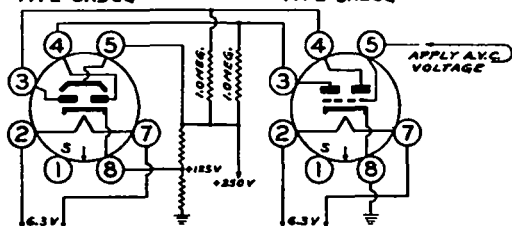
CONTROL TUBE TYPE 6AE6G
