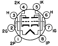
BASING DIAGRAM JEDEC 8DG
