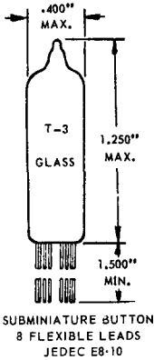
OUTLINE DRAWING JEDEC 3-11
