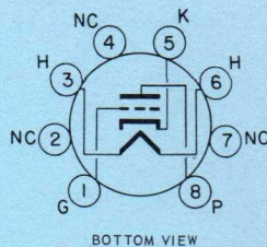
OUTLINE DRAWING JEDEC 8DK
