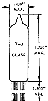
SUBMINATURE BUTTON 8 FLEXIBLE LEADS JEDEC E8-10
