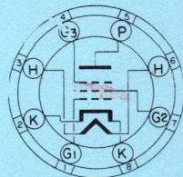
BOTTOM VIEW SUBMINIATURE BUTTON
