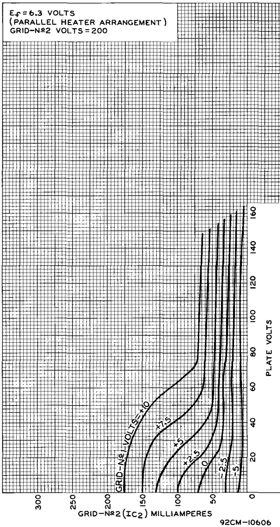
Fig.5 - Average Grid-No.2 Characteristics for Each Pentode of Type 6939.
