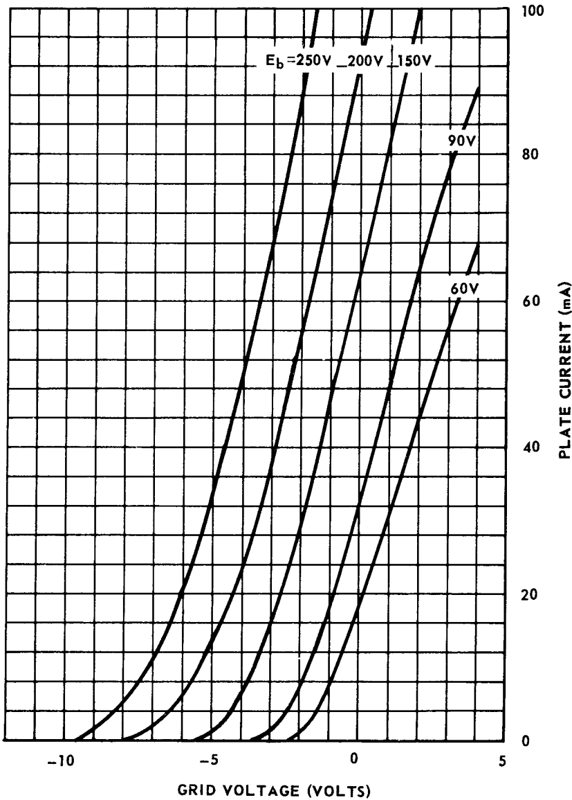
TRANSFER CHARACTERISTICS
