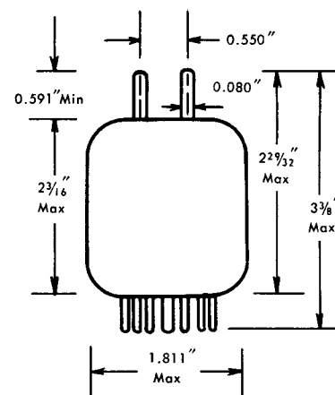
OUTLINE DRAWING
