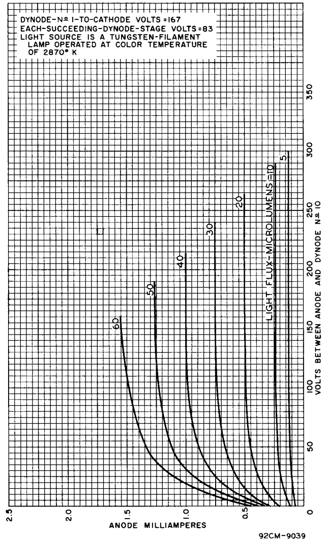
Fig. 4 - Average Anode Characteristics of Type 6903.
