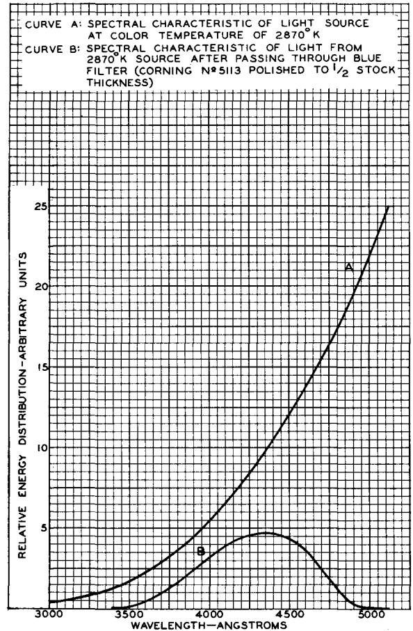
Fig. 2 - Spectral Characteristic of 2870°K Light Source, and Spectral Characteristic of Light from 2870°K after Passing through Indicated Filter.
