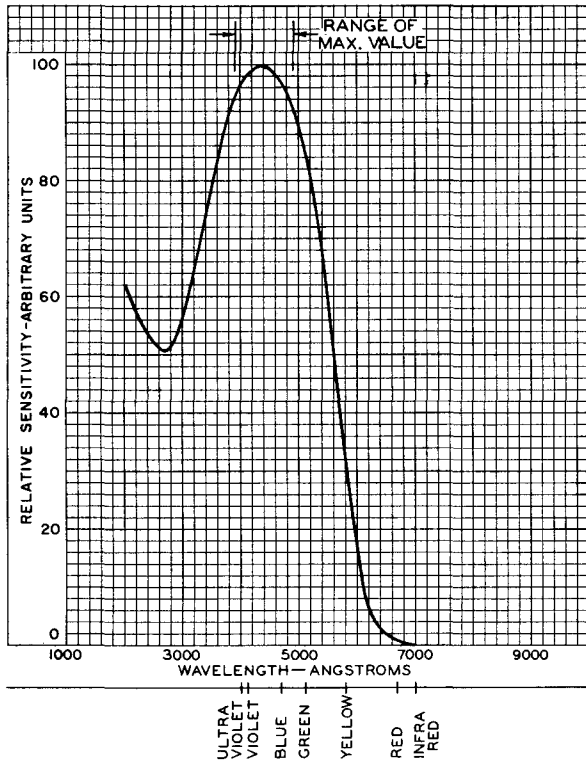
Fig. 1 - Tentative Spectral Sensitivity Characteristic of Type 6903 which has S-13 Response. Curve is shown for Equal Values of Radiant Flux at All Wavelengths.
