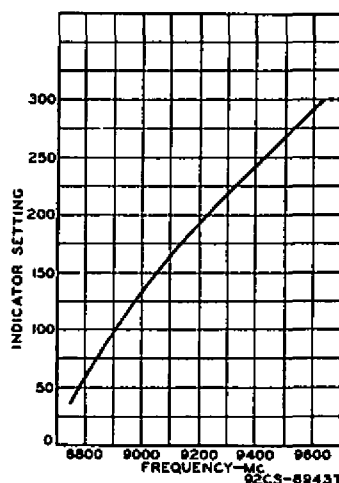
Fig. 4 - Typical Tuning Characteristic of Type 6865.
