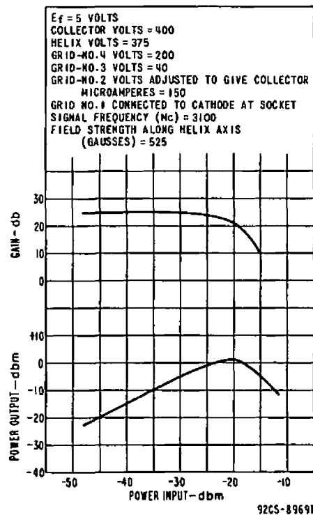
Fig. 10 - Saturation Characteristics of Type 6861.
