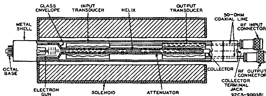
Fig.1 - Schematic Arrangement of Type 6861 with Associated Solenoid.
