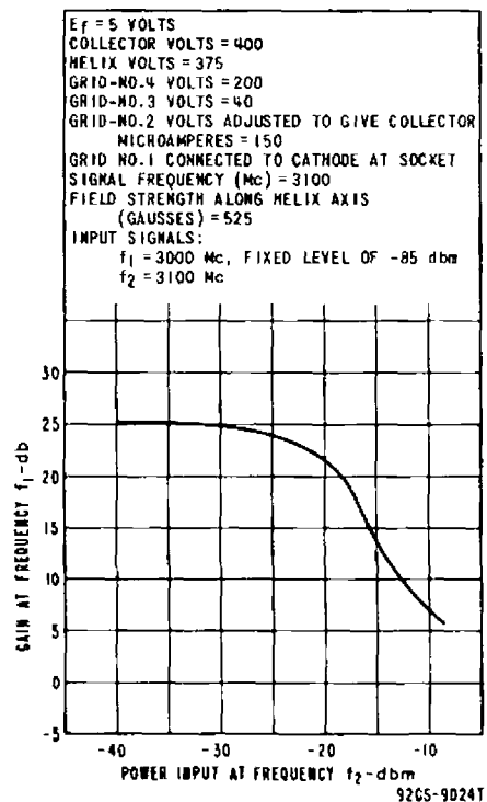
Fig. 13 - Cross-Modulation Characteristic of Type 6861.
