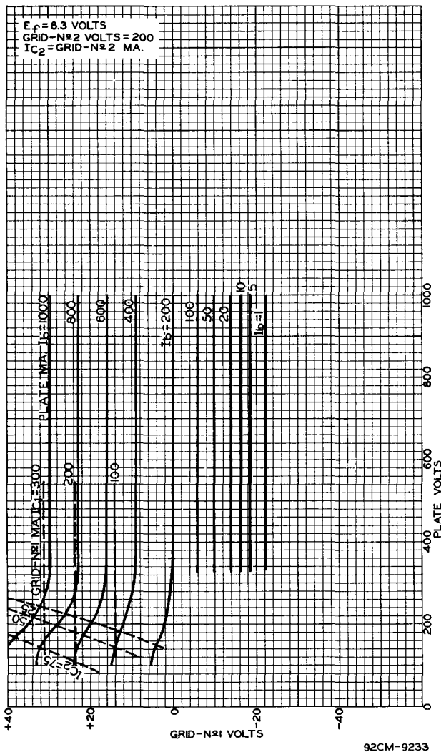
Fig. 10 - Typical Constant-Current Characteristics of Type 6816.
