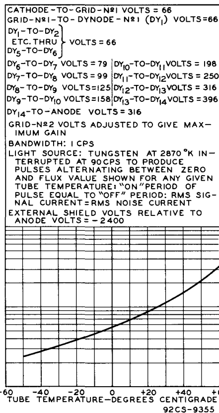
Fig.10 - Equivalent-Noise-Input Characteristic of Type 6810-A Used in High-Output-Pulse Service.
