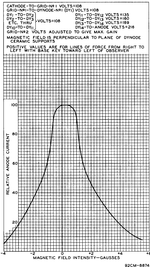
Fig.12 - Effect of Magnetic Field on Anode Current of Type 6810-A Used in Low-Light, Low-Noise, High-Gain Service.
