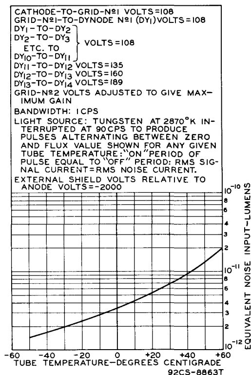
Fig.9 - Equivalent-Noise-Input Characteristic of Type 6810-A Used in Low-Light, Low-Noise, High-Gain Service.
