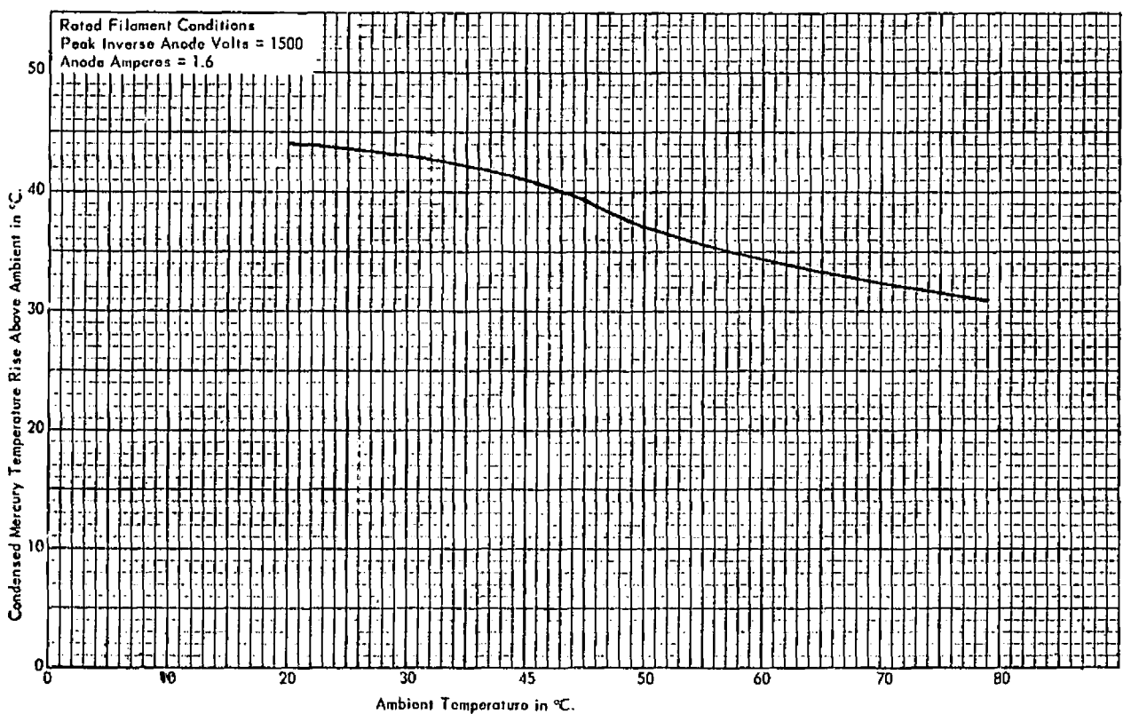
CONDENSED MERCURY TEMPERATURE RISE ABOVE AMBIENT AS A FUNCTION OF AMBIENT TEMPERATURE
