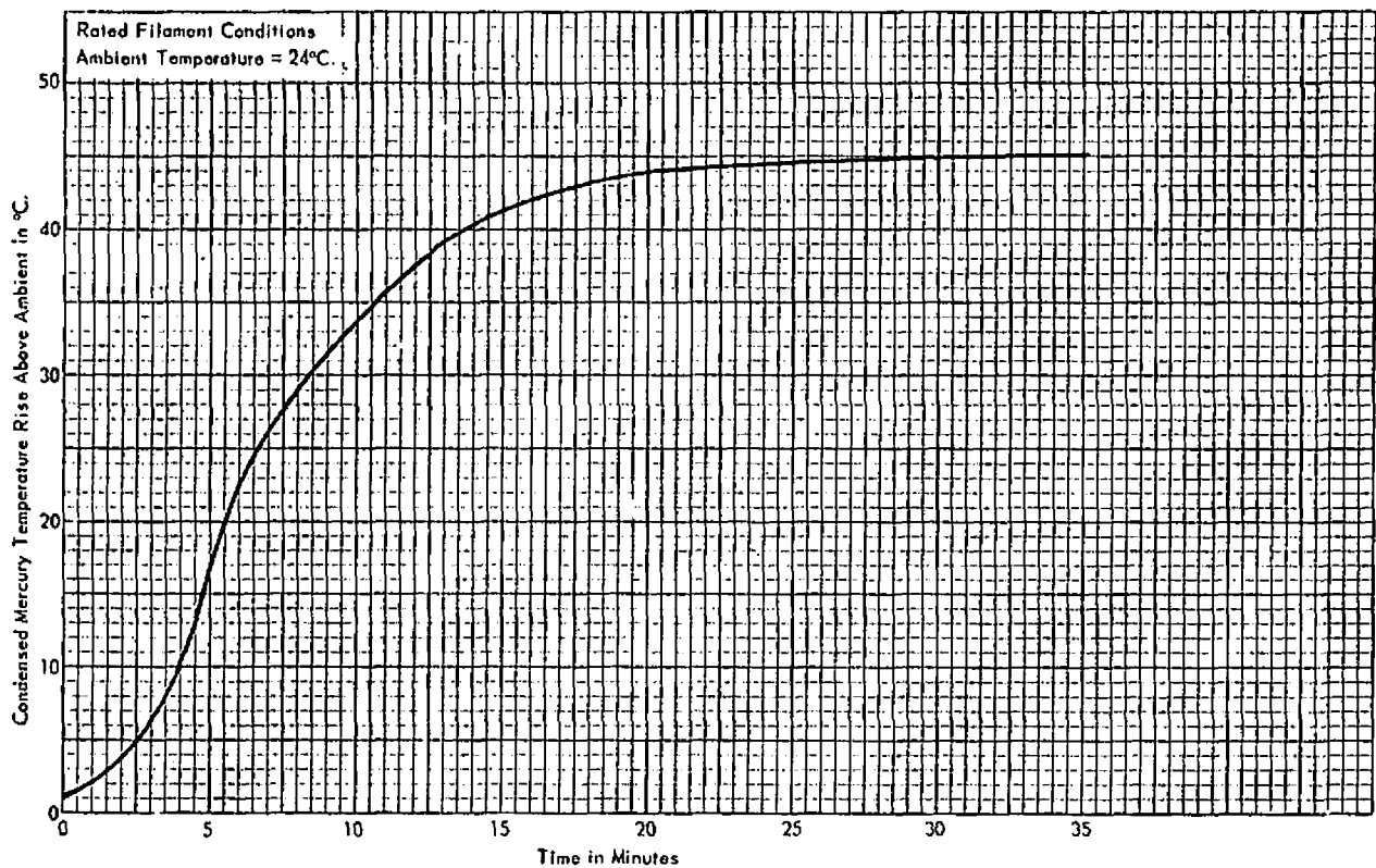
RATE OF CONDENSED MERCURY TEMPERATURE RISE ABOVE AMBIENT
