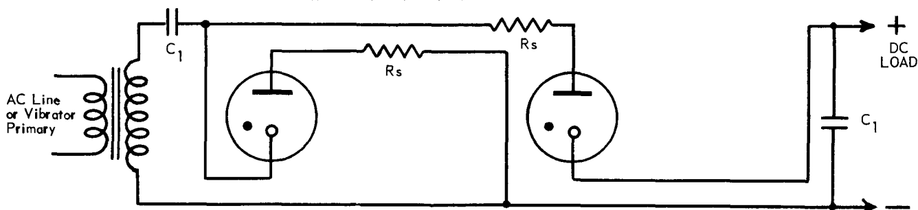
VOLTAGE DOUBLER HIGH VOLTAGE POWER SUPPLY TYPICAL CIRCUIT FOR AC LINE OR BATTERY OPERATION
