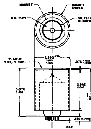
Figure 1 Outline Drawing
