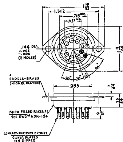
Figure 3 Contact Socket Assembly
