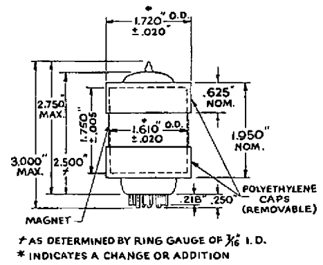
Figure 1 Outline Drawing
