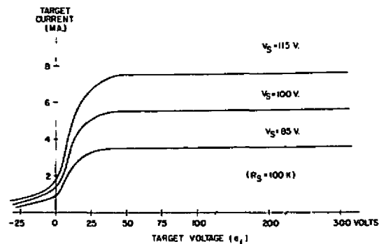
Figure 4 Output characteristic
