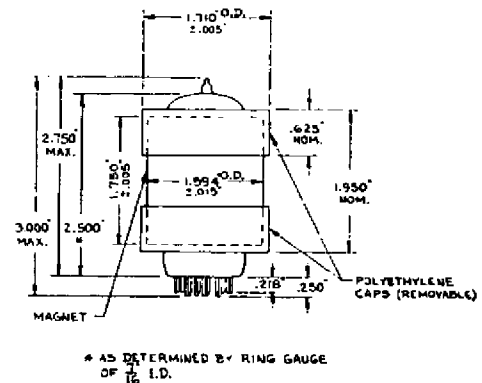
Figure 1 Outline Drawing
